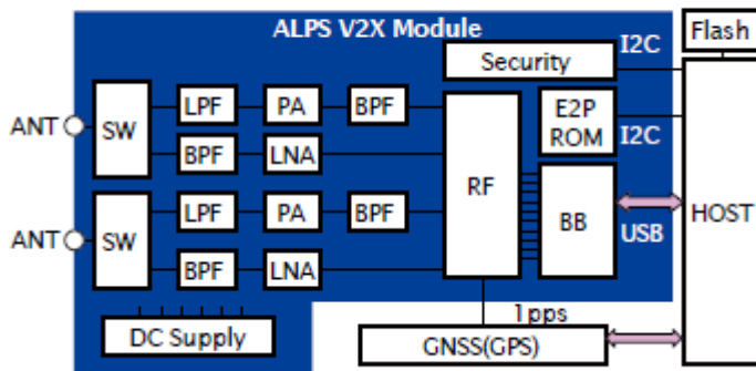
V2X system block diagram
